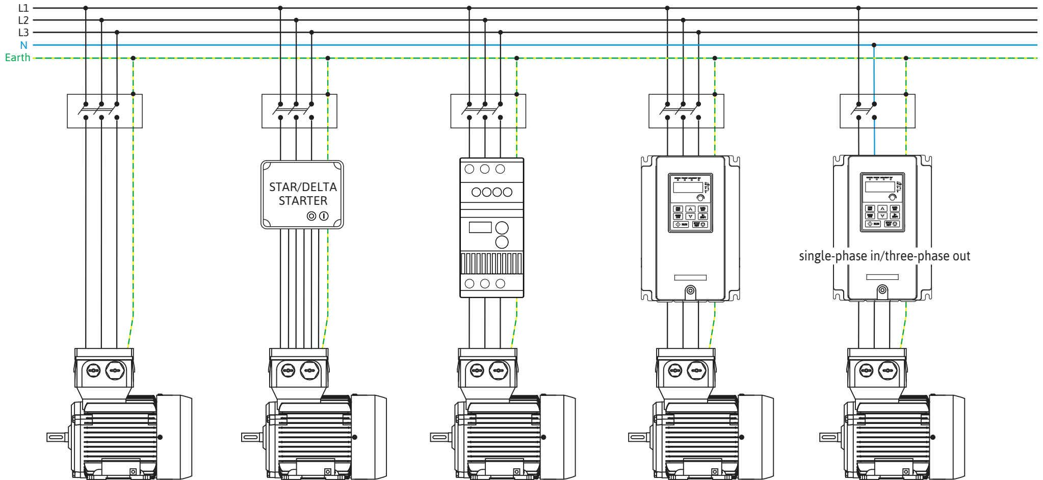
DOL (Direct On Line) Motor wound in STAR or DELTA for Mains Voltage
